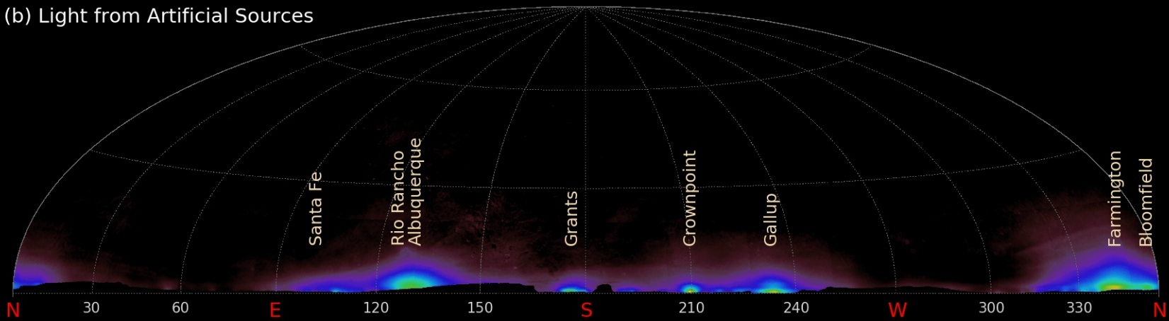
Figure 12: Panoramic night sky images from the Water Tank site on 05/30/2008. (a) Observed night sky. (b) Light from artificial sources.
